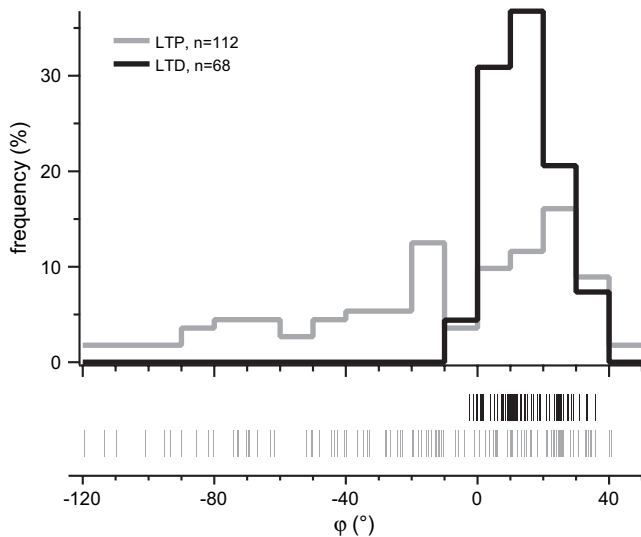
Fig. 6. A histogram of \phi for our entire data set of LTP and LTD experiments (excluding those conducted in the presence of pharmacological agents). Each vertical line in bottom graph denotes an experiment carried out using one unitary L5-to-L5 connection. Note that this figure includes a re-analysis of previously published LTD and LTP experiments (Sjöström et al., 2001, 2003, 2004; Watt et al., 2004) in addition to the data included in this paper. LTD induction protocols included post-before-presynaptic firing at 0.1–20 Hz as well as pairing of presynaptic firing at 0.1–30 Hz with postsynaptic subthreshold depolarization. LTP induction protocols included pre-before-postsynaptic firing at 0.1–100 Hz, or pre- and postsynaptic depolarizing current pulses as in Fig. 1.
