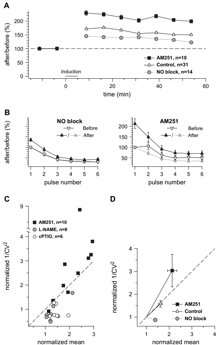
Fig. 5. Pharmacological dissection of LTP. (A) LTP induced under control conditions (open triangles; same data as in Fig. 1B), in the presence of the endocannabinoid inhibitor AM251 (closed squares), or during NO signaling blockade (closed gray circles; pooling results obtained using the NO synthase inhibitor L-NAME and the NO scavenger cPTIO). (B) Left panel: Short-term plasticity before and after LTP induction during NO blockade (L-NAME and cPTIO results pooled). Right panel: Short-term plasticity before and after LTP induction in the presence of AM251. (C) CV analysis of individual LTP experiments in the presence of AM251, L-NAME, or cPTIO. (D) Average change in 1/CV^2 following LTP induction under the conditions indicated in C. Note that CB1 blockade (AM251) increases both the amount of LTP and the degree of presynaptic expression, whereas NO blockade reduces the amount of LTP while at the same time rendering the locus of expression completely postsynaptic.
